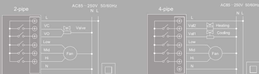
Wiring Diagram
